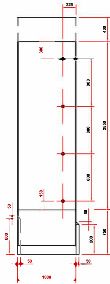
R/H Full Corner
