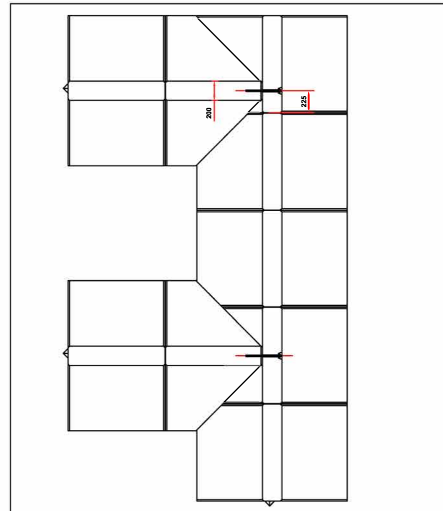
L/H Full Corner
